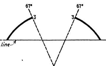
FIG. 13.—Basal plane (00·1) diffraction arcs. X-ray beam 8° to rolling plane, 50° to rolling direction.
